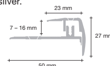
Stair nose, aluminium PGSTPSILVME270N, 2700 x 23 mm Fits flooring thickness of 7 – 16 mm. Surface: aluminium. Colour: silver.
